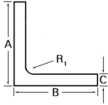
Square toes x 20ft Canadian Profile
